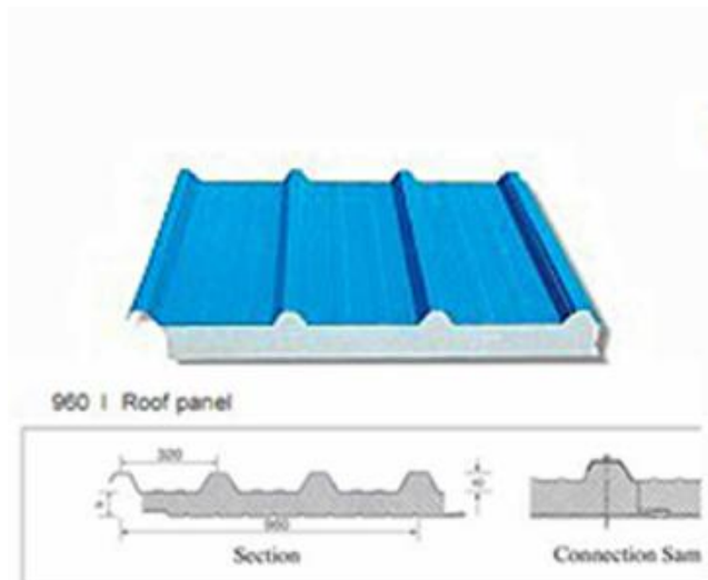
EPS sandwich panel for roof
