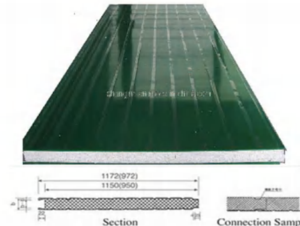
EPS sandwich panel for wall
